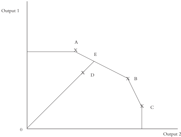
Figure 1. Data envelopment analysis.
